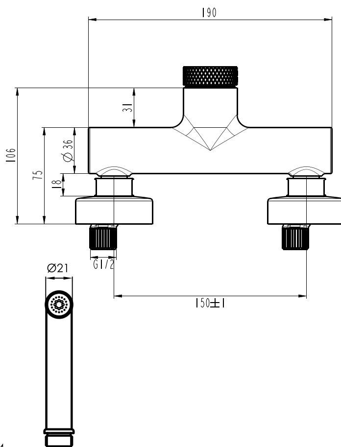
Front View
